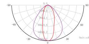
Optical options: 30°*90°
